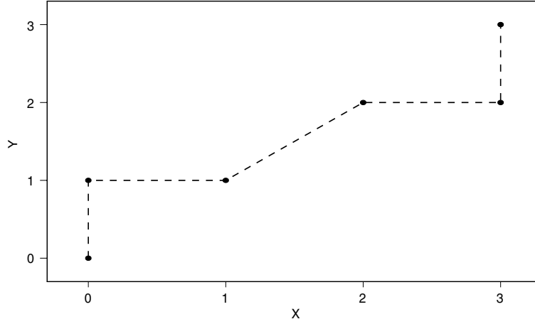
Figure 2: A discrete example
