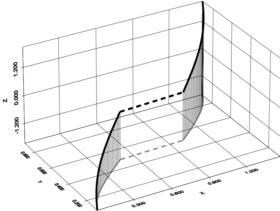
Figure 1: A continuous example with n = 3 .
