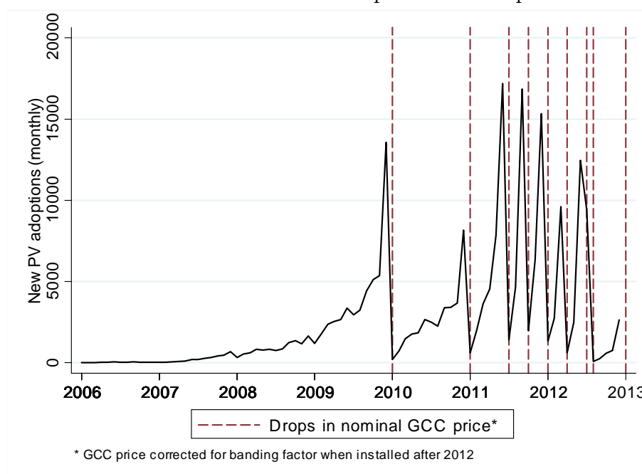
Figure 3: 2006-2012: Time series of new PV adoptions and drops in nominal GCC price
